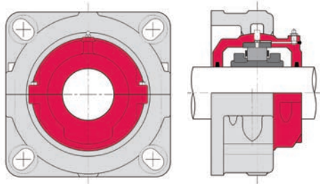
SQUARE (DF) FLANGE
