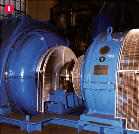
1. Coal industry mine winders include 03 Series 600mm for an operating load of 80 tonnes per bearing at 48 rpm and 02 Series 400mm for an operating load of 32 tonnes per bearing at 31 rpm.
